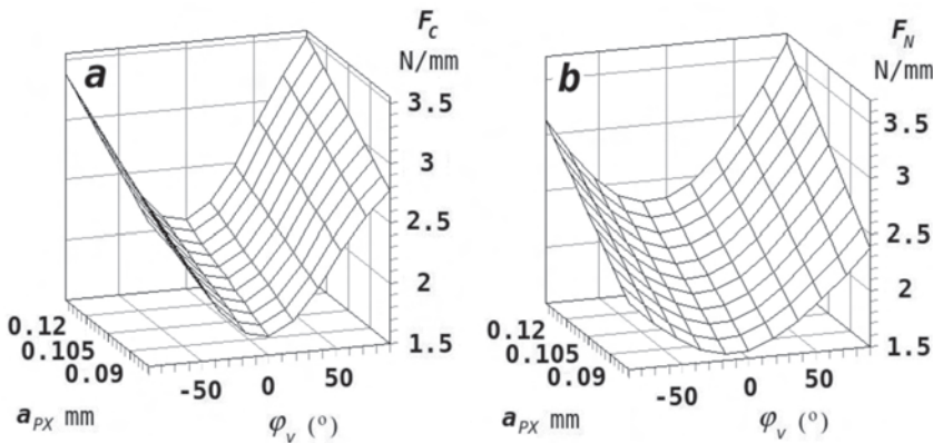
Figure 14. Plot of: a) main F_C , and b) normal F_N , cutting forces vs. grain orientation angle \phi_V , and maximum chip thickness a_{px} , according to equations (1) and (2) for down-routing of the Douglas fir ( Pseudotsuga menziesii ).
