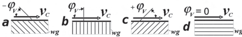
Figure 1. Wood cutting: a : against the grain; b : perpendicular the grain; c : along the grain; d : parallel to grain; wg = wood grain orientation.
