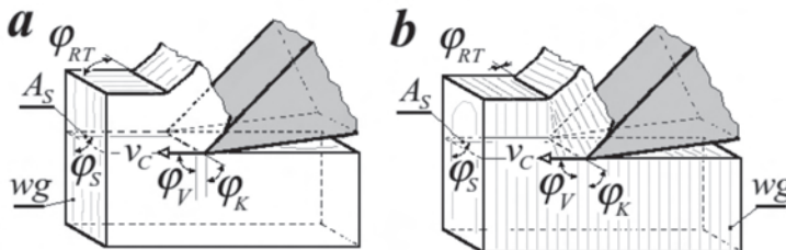
Figure 3. Orientation angles between wood grain ( wg ) and: v_c - vector of cutting velocity; k - cutting edge; A_s - cutting plane; for perpendicular cutting case ( \varphi_k=90^\circ , \varphi_v=90^\circ , \varphi_s=90^\circ ); by growth rings orientation angle \varphi_{RT} : a - \varphi_{RT}=90^\circ (radial); b - \varphi_{RT}=0^\circ (tangential); A_s - cutting plane.
