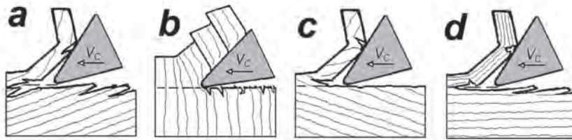
Figure 2. Chip and fractures formation during cutting: a : against grains grain ( \varphi_k=90^\circ , \varphi_v=-20^\circ , \varphi_s=-20^\circ ); b : perpendicular ( \varphi_k=90^\circ , \varphi_v=90^\circ , \varphi_s=90^\circ ); c : with the grain ( \varphi_k=90^\circ , \varphi_v=20^\circ , \varphi_s=20^\circ ); d : parallel ( \varphi_k=90^\circ , \varphi_v=0^\circ , \varphi_s=0^\circ ).
