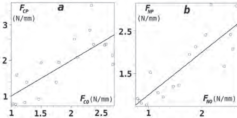
Figure 9. For down-routing routing of Oak ( Quercus petraea ): a) plot of the main cutting force observed F_{CO} against the main cutting force predicted F_{CP} according to equation (3), b) plot of the normal force observed F_{NO} , against normal force predicted F_{NP} , according to equation (4).
