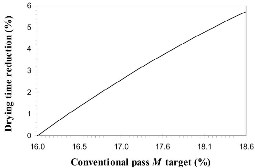
Figure 10: Reduction in drying time with respect to the base case.
