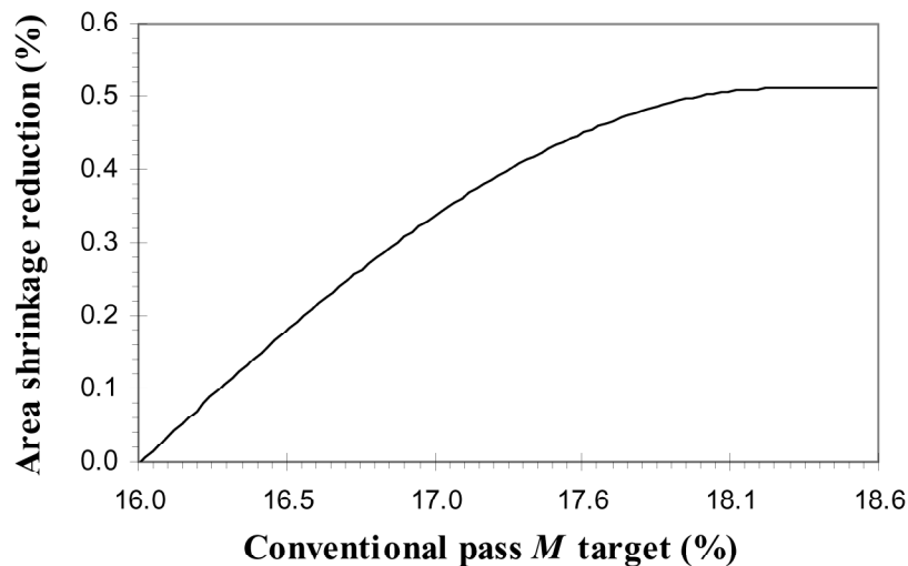
Figure 9: Reduction in area shrinkage with respect to the green timber.
