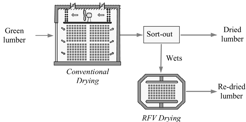
Figure 2: General diagram of the dry-sort-redry strategy.
