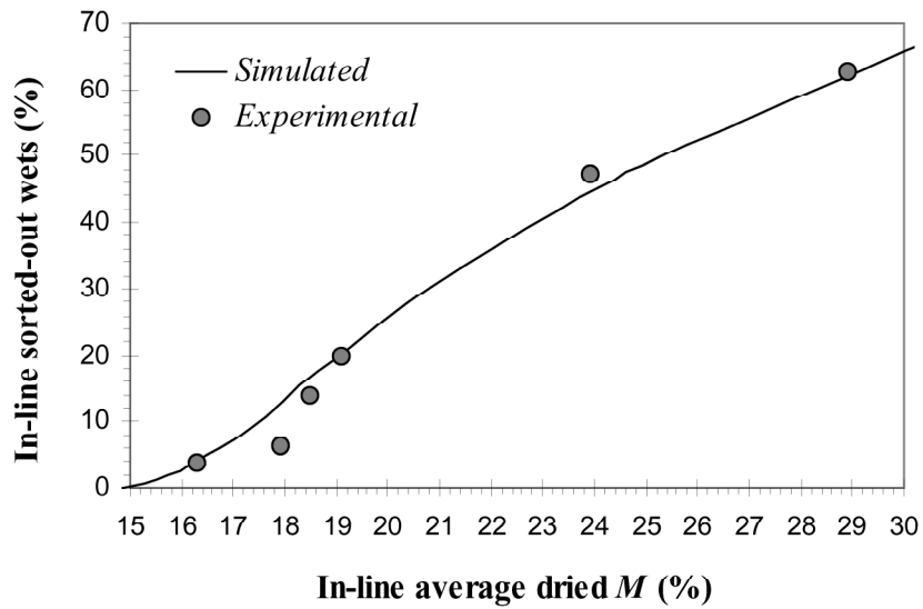
Figure 5: Simulated and experimental percentages of wets as function of the average M .
