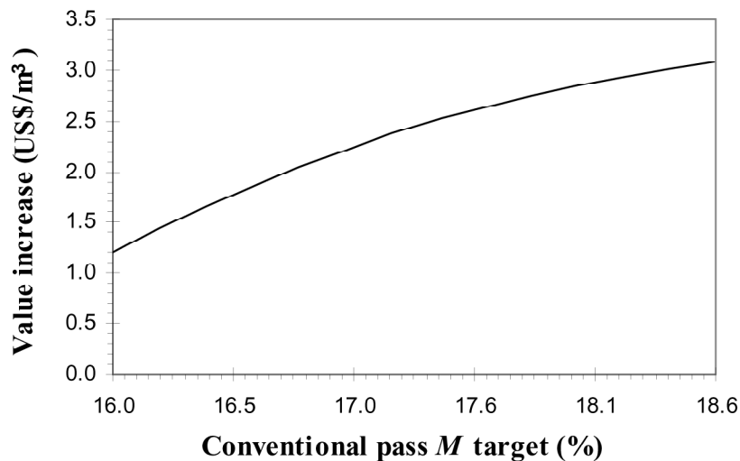
Figure 11: Increase in timber value with respect of the base case.
