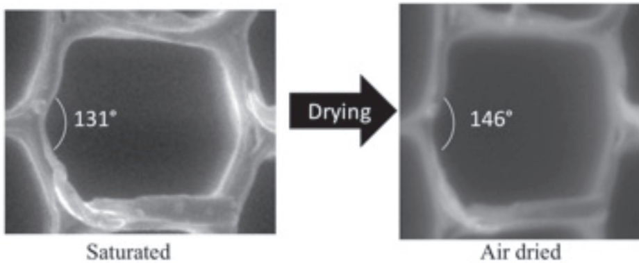
Figure 6. Zoom of an earlywood tracheid showing the change of cell wall shape caused by drying.
