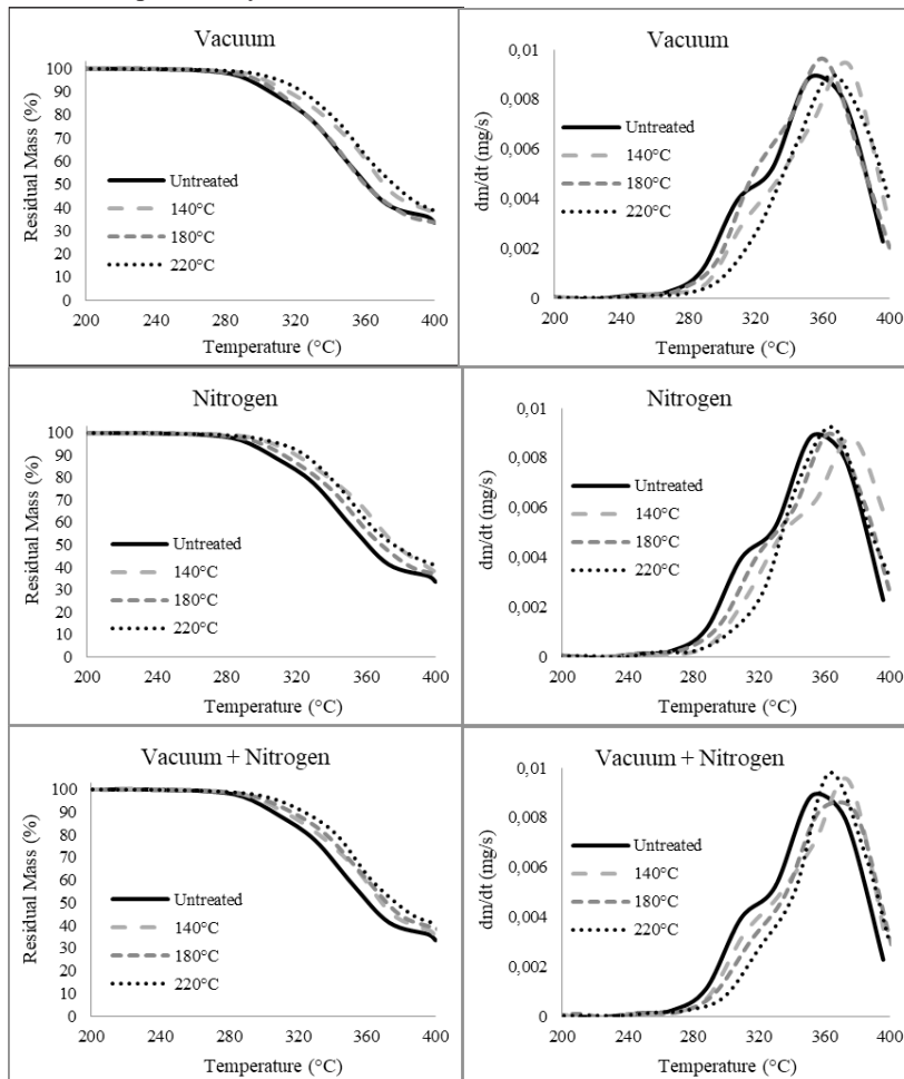
Figure 1: Graphs obtained from the thermogravimetric analysis (TGA) and the respective thermogravimetric derivative (DTG) of thermally treated Eucalyptus grandis woods at different temperatures - 140, 180 and 220°C - as a function of the treatment atmosphere condition.
