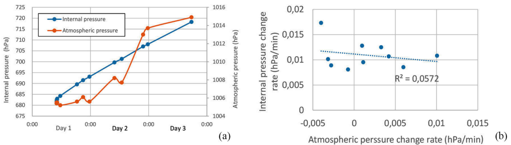
Figure 9: Relationship between internal pressure and atmospheric pressure. (a) changes in the internal and atmospheric pressures (b) relationship between atmospheric pressure change rate and the internal pressure change rate.
