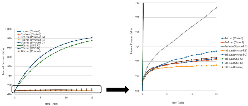
Figure 7: Relationship between time and the internal pressure in the panel specimen experiment.
