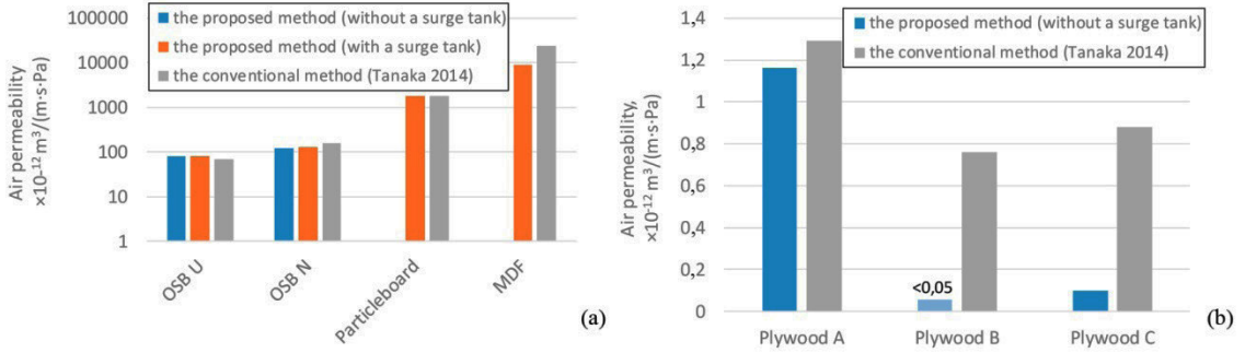
Figure 8: Air permeability of the testing panels. (a) results of OSB, particleboard and MDF (b) results of plywood.
