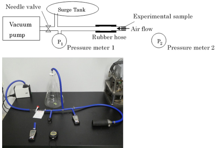
Figure 4: Schematic and photograph of the measurement system with a surge tank.
