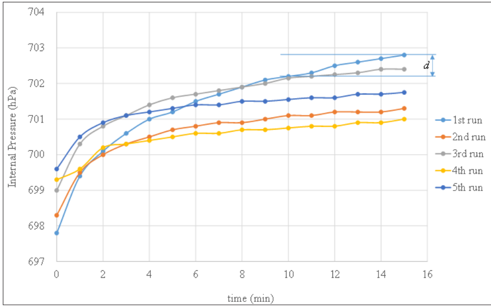
Figure 5: Relationship between time and the internal pressure of the system in the control specimen experiment (Day 1).
