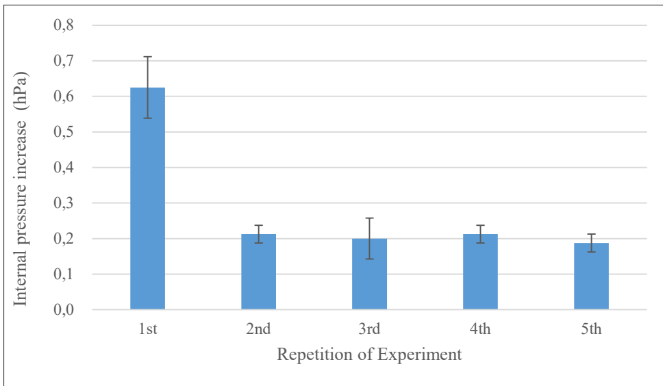
Figure 6: Influence of the repetition (1 st -5 th runs) of the control specimen experiment on the internal pressure increase from t = 10 to t = 15 .
