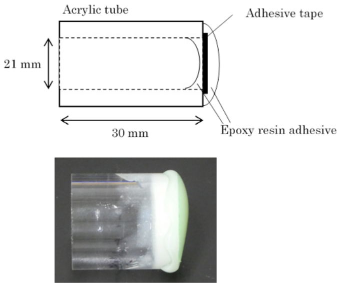
Figure 2: Schematic and photograph of the control specimen.
