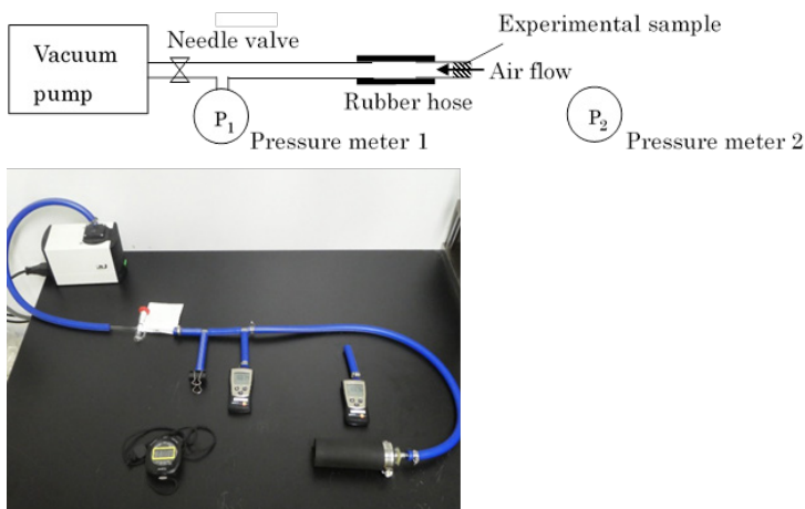
Figure 3: Schematic and photograph of the measurement system.
