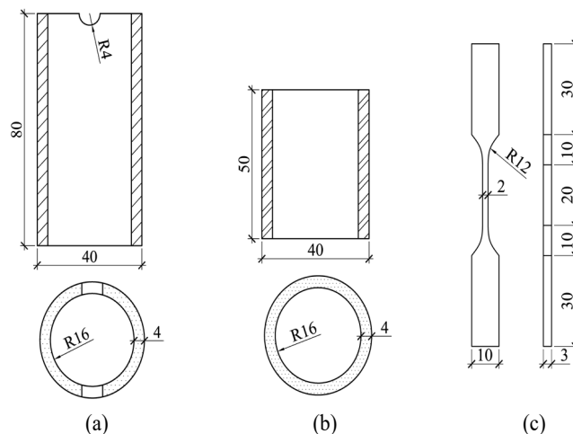
Figure 3: Configurations of samples used in this study (a) half-hole bolt-bearing sample, (b) compression sample, and (c) tension sample.
