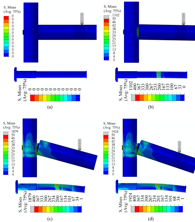
Figure 14: Stress distributions of bamboo-bolt joint during bending load processes a) initial state, b) preliminary load state, c) maximum load state and d) failure state.
