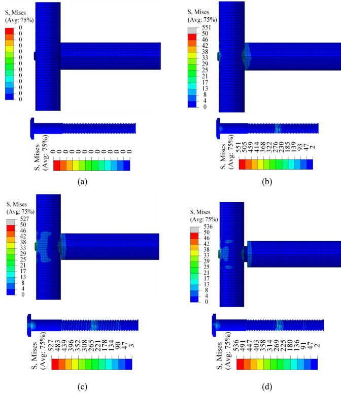
Figure 13: Stress distributions of bolted bamboo joint during withdrawal load processes a) initial state, b) preliminary load state, c) maximum load state and d) failure state.
