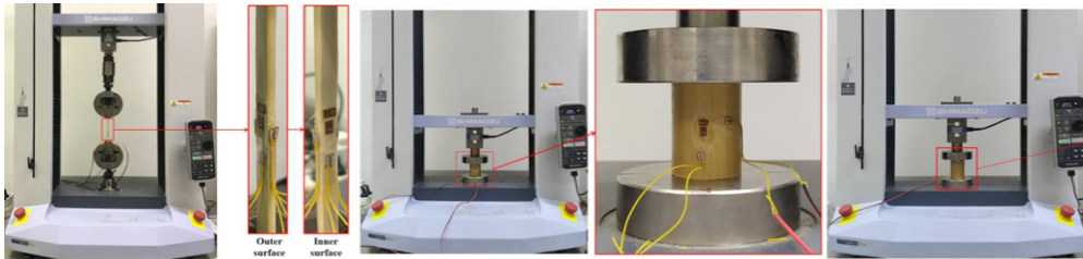
Figure 7: Setups for measuring elastic modulus and Poisson’s ratio of Moso bamboo (a) tension method, (b) compression method, and (c) bolt-bearing method.
