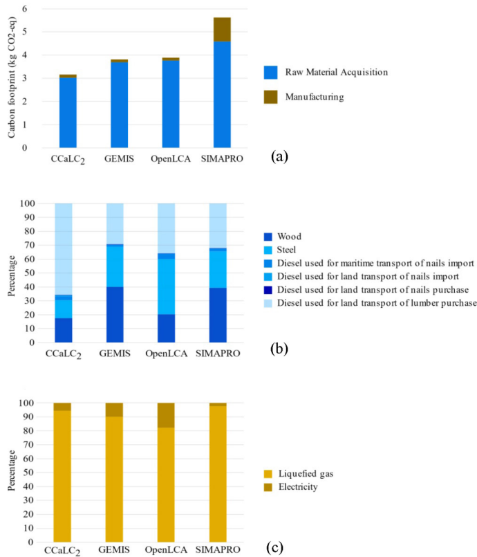
Figure 1: (a) Total carbon footprint of the wooden pallet obtained by each software studied, and (b) the percentage contribution of the process to raw material acquisition and (c) manufacturing.
