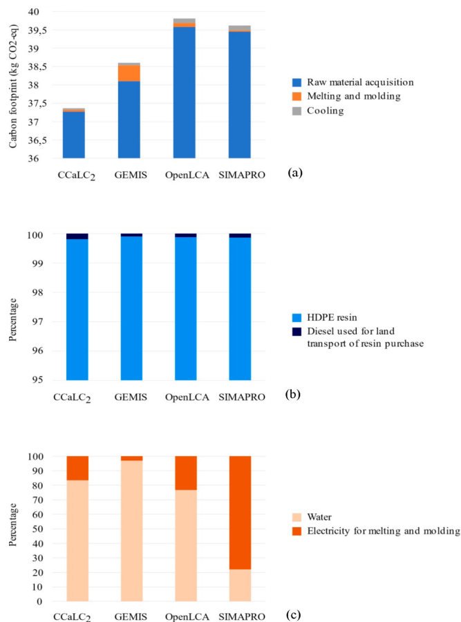
Figure 2: (a) Total carbon footprint of the plastic pallet obtained by each software studied, and (b) the percentage contribution of the process to raw material acquisition, (c) melting and molding stage.
