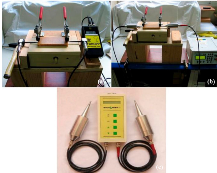
Figure 1: (a) Stress wave test (b) Ultrasound test USLab (c) Ultrasound Sylvastest.
