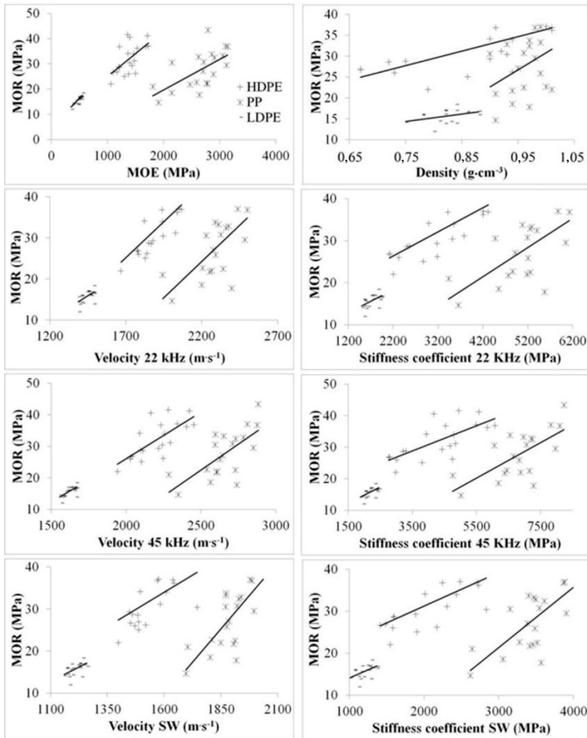
Figure 4: MOR of the specimens as a function of MOE, density, wave velocity, stiffness coefficient, with regression lines for each group of composites of the same matrix (= LDPE; +HDPE; *PP).
