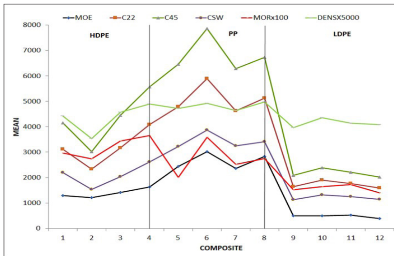
Figure 2: Trend line graph for density, MOE, MOR, and stiffness coefficient of the different composites.
