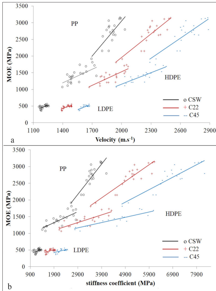
Figure 3: MOE as a function of the a) wave velocity and b) stiffness coefficient with the regression line for each composite group with the same matrix.
