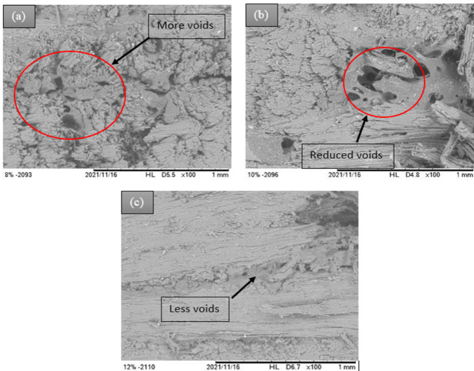
Figure 4: Cross section - SEM (Zoom 100x): (a) 8 %; (b) 10 %; (c) 12 %.
