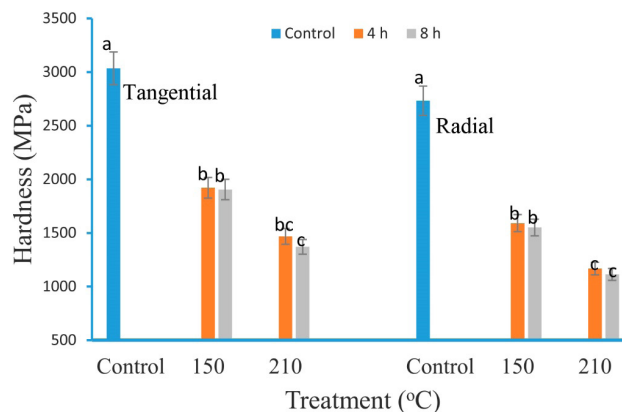
Figure 2: Brinell hardness of tin alloy thermal modified Chinese bottletree ( Firmiana simplex (L.) W. Wight) wood.
