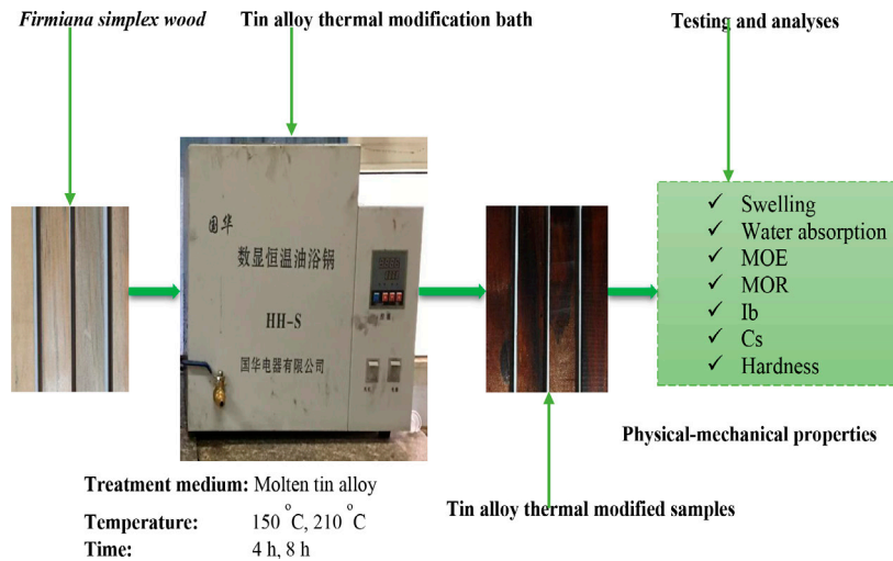
Figure 1: Schematic diagram of tin alloy thermal modification experiment.
