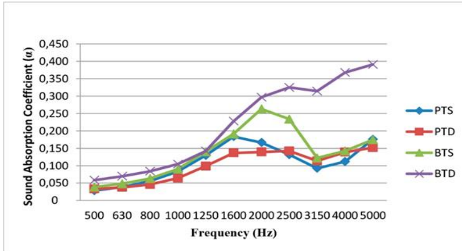
Figure 7: Comparison of the samples of the tangent cutting direction. (PTS: Pine-Targett-Single Comp., PTD: Pine- Targett -Double Comp BTS: Beech- Targett -Single Comp., BTD: Beech- Targett -Double Comp.)
