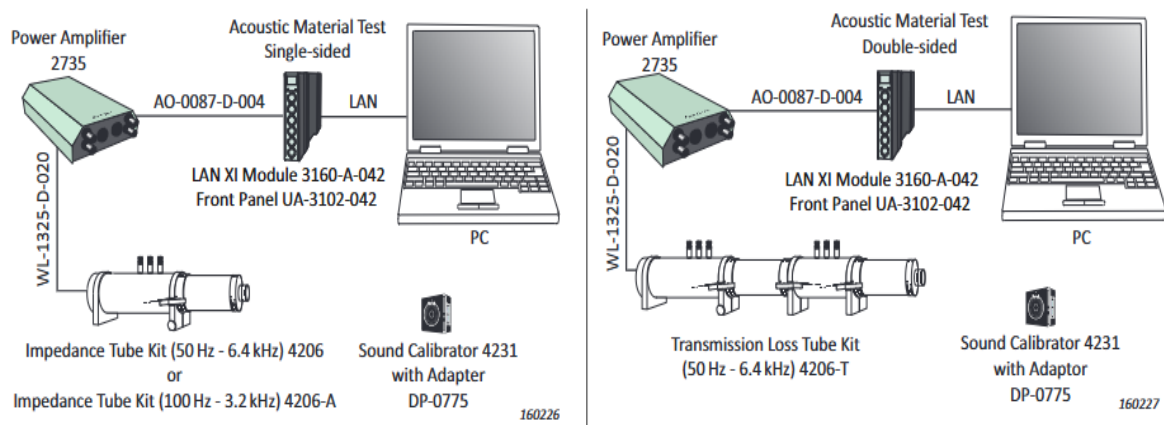
Figure 4: The physical layer of the analyzed system (Brüel and Kjaer 2024).
