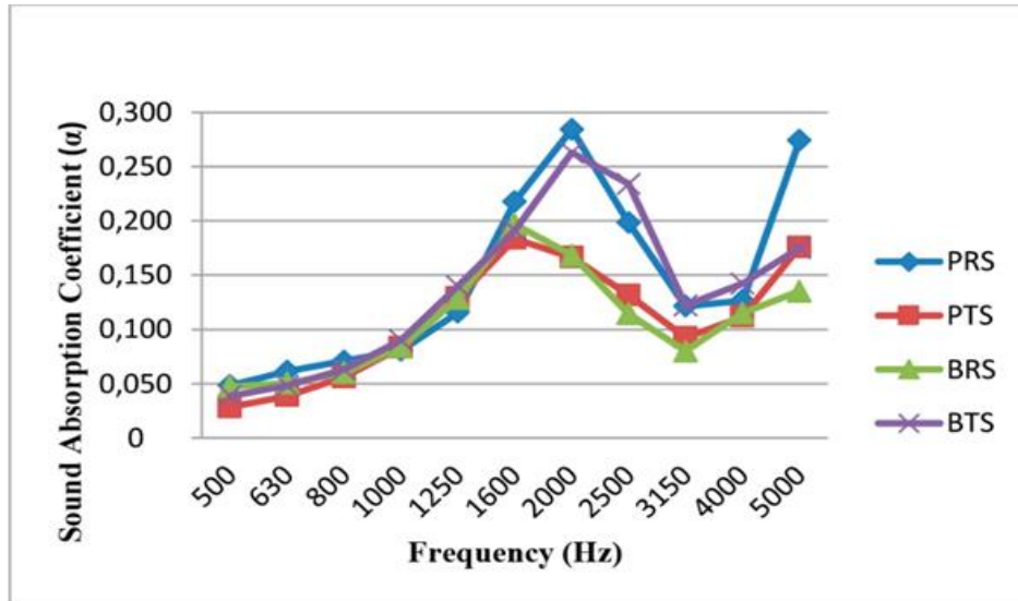
Figure 8: Comparison of samples of one component varnish. (PRS: Pine-Radial-Single Comp. PTS: Pine-Tangent-Single Comp. BRS: Beech-Radial-Single Comp. BTS: Beech-Tangent-Single Komp.)
