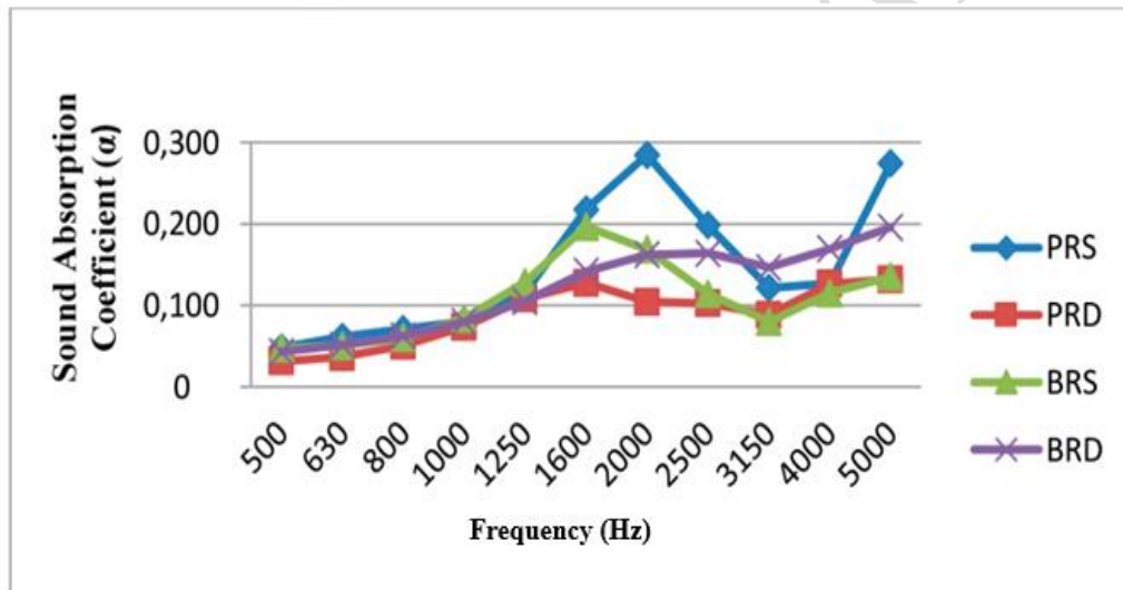
Figure 6: Comparison of the samples of the radial cutting direction. (PRS: Pine-Radial-Single Comp., PRD: Pine-Radial-Double Comp. BRS: Beech-Radial-Single Comp., BRD: Beech-Radial-Double Comp)
