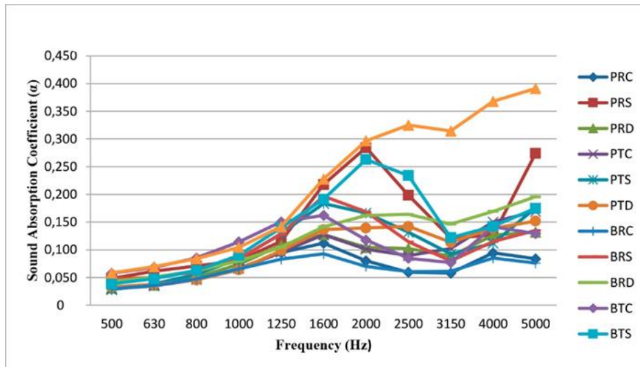
Figure 10: Wood type-cutting direction-varnish type comparison.
