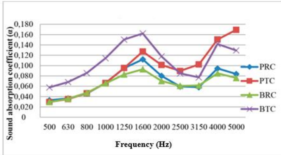
Figure 5: Comparison of control samples of wood material type.
