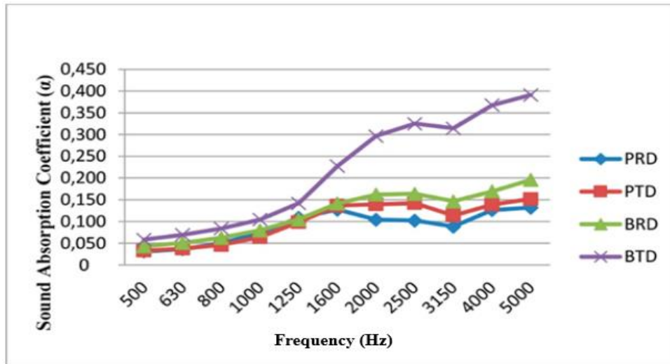
Figure 9: Comparison of samples of double component varnish. (PRD: Pine-Radial-Double Comp. PTD: Pine-Target- Double Comp. BRD: Beech-Radial- Double Comp. BTD: Beech-Target- Double Comp.)
