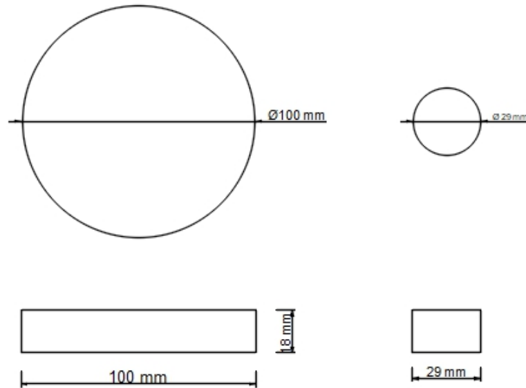
Figure 1: Cutting dimensions of the test samples.
